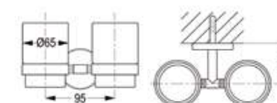
RAK21014 Double tumbler holder, glass wall fastening with screws and dowels
