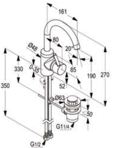
RAK12028 Side Single lever basin mixer DN 15 ceramic cartridge-K35 with swivelling spout cache aerator M 16.5 x 1 1/2" high pressure flexible hose with PEX tubes pop up waste 1 1/4 European standard- EN 817
