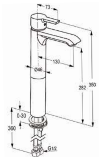
RAK13061 single lever basin mixer XL HR DN 15 ceramic cartridge-K35 aerator M 24 x 1 1/2" high pressure flexible hose with PEX tubes European standard - EN 817
