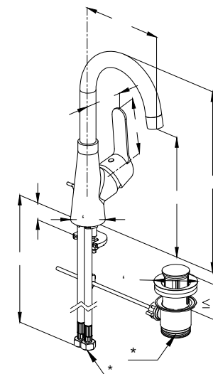
RAK18028 Side Single lever basin mixer DN 15 ceramic cartridge - K35 aerator M 24 x 1 1/2" high pressure flexible hose with PEX tubes pop up waste 1 1/4 inch European Standard- EN 817
