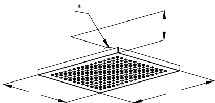
RAK22056 ABS Over head shower DN 15 260 mm x 200 mm with cleaning system with ball joint connection 1/2 inch
