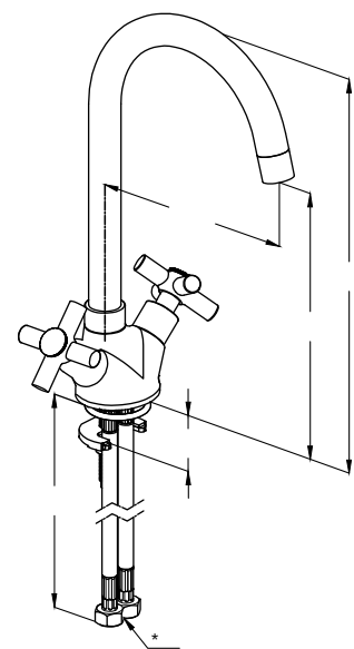
RAK34000 Dual controlled sink mixer DN15 deck mounted with swivel spout aerator M22 x 1 1/2"high presssure flexible hose with PEX tubes European Standard - EN 200
