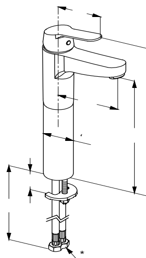
RAK18061 single lever basin mixer XL HR DN 15 ceramic cartridge-K35 aerator M 24 x 1 1/2" high pressure flexible hose with PEX tubes European standard - EN 817
