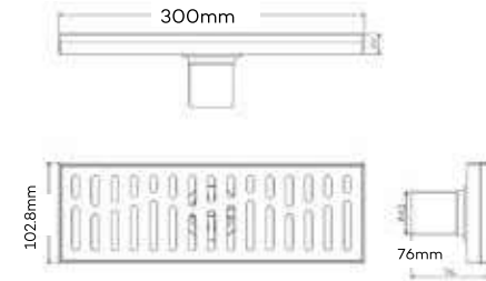
RAK90730 Floor Drain Long Grate Insert with Smell Prevention Cover Type A Channel 300x103mm SS 304 Satin finish
