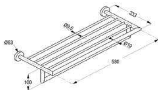
RAK91020 Shelf with Towel Bar 580mm SS 304 Satin finish
