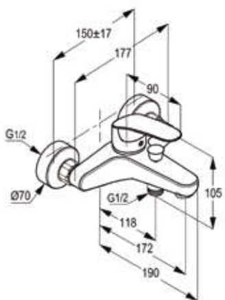
RAK17002 Single lever bath & shower mixer DN 15 without shower set ceramic cartridge-K35 aerator M 24 X 1 flow class CB automatic diverter: shower to bathtub shower outlet G 1/2" protected against back flow S- unions 1/2 X 3/4 inch European standard- EN 817
