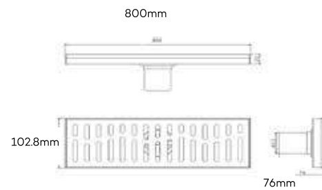
RAK90732 Floor Drain Long Grate Insert with Smell Prevention Cover Type A Channel 800x103mm SS 304 Satin finish
