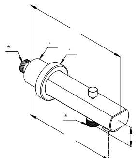
RAK11013 PROJECT wall spout DN15 aerator M 28 x 1 flow class BB automatic diverter: shower to bathtub shower outlet 1/2 inch protected against back flow with sliding cover plate Ø 60 mm projection 170 mm Available Finishes
