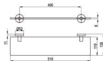
RAK91010 Glass Shelf 519mm SS 304 Satin finish & Glass
