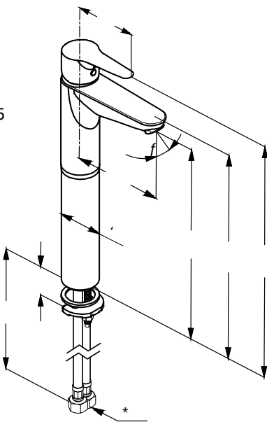
RAK10061 single lever basin mixer XL HR DN 15 ceramic cartridge-K35 aerator M 24 x 1 1/2" high pressure flexible hose with PEX tubes European standard - EN 817
