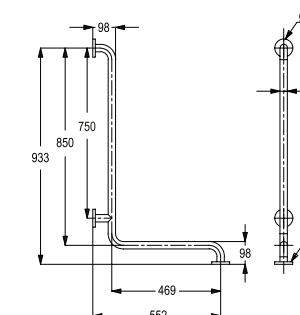
RAK90420 Grab Bar Horizontal Angled SS 304 Satin finish
