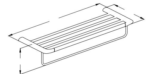
RAK20020 Towel shelf with towel bar wall fastening with screws and dowels
