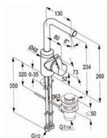
RAK13028 Side Single Lever Basin Mixer DN 15 ceramic cartridge-K35 swivelling spout-(360 °) PCA cache aerator M 16.5 x 1 1/2" high pressure flexible hose with PEX tubes pop up waste 1 1/4 inch European Standard - EN 817
