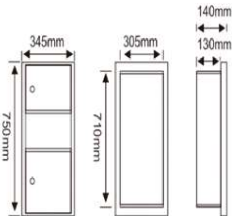
RAK90511 Paper Towel Dispenser with Waste Receptacle, Recessed Capacity up to 350C-fold or 475 multifold Waste container capacity 7L Two doors with front tumbler locks keyed SS 304 Satin finish
