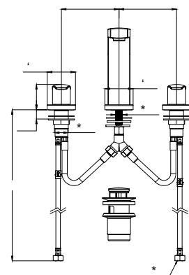
RAK17041 basin mixer DN 15 3 hole deck mounted solid levers ceramic head part 90°, Right and Left flexible high pressure supply tubes 1/2 inch PCA aerator M 24 x 1 rapid installation set click clack
