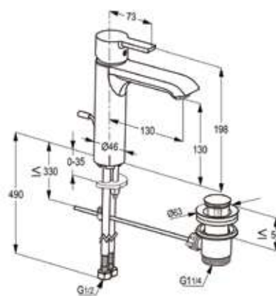
RAK13060 Single lever basin mixer XL DN 15 ceramic cartridge - K35 aerator M 24 x 1 1/2" high pressure flexible hose with PEX tubes pop up waste 1 1/4 inch European Standard - EN 817
