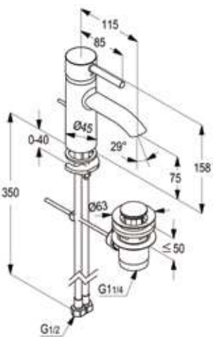
RAK12000 Single lever basin mixer DN 15 ceramic cartridge-K35 cache aerator M 16.5 x 1 1/2" high pressure flexible hose with PEX tubes pop up waste 1 1/4 inch European Standard - EN 817
