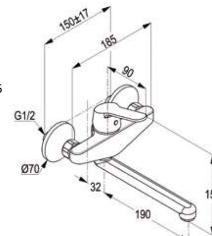
RAK18008 Wall mounted single lever sink mixer DN 15 ceramic cartridge-K35 swivelling (185°) spout l = 200 mm aerator M 24 x 1 flow class A S- unions 1/2 X 3/4 inch European standard- EN 817
